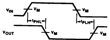
Waveform 1. Waveform For Inverting Outputs
