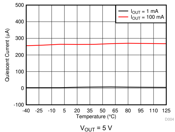
Figure 5-4. Quiescent Current vs Ambient Temperature
