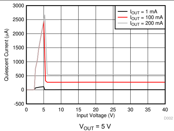
Figure 5-2. Quiescent Current vs Input Voltage
