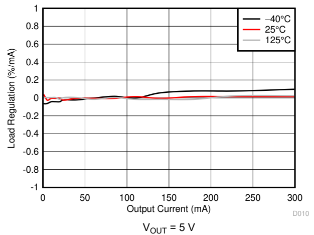
Figure 5-10. Load Regulation
