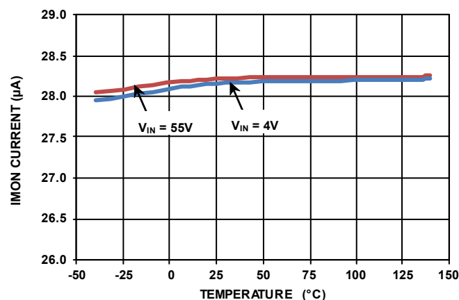
FIGURE 37. IMON OUTPUT CURRENT ACCURACY (CURRENT-SENSING SIGNAL OUTPUT) vs TEMPERATURE, V_{SENx} = 30mV , R_{SETx} = 665\Omega (0.1%)
