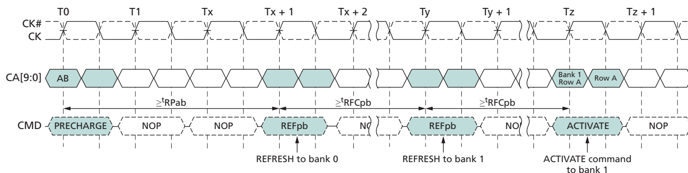
Figure 59: Per-Bank REFRESH Operation
