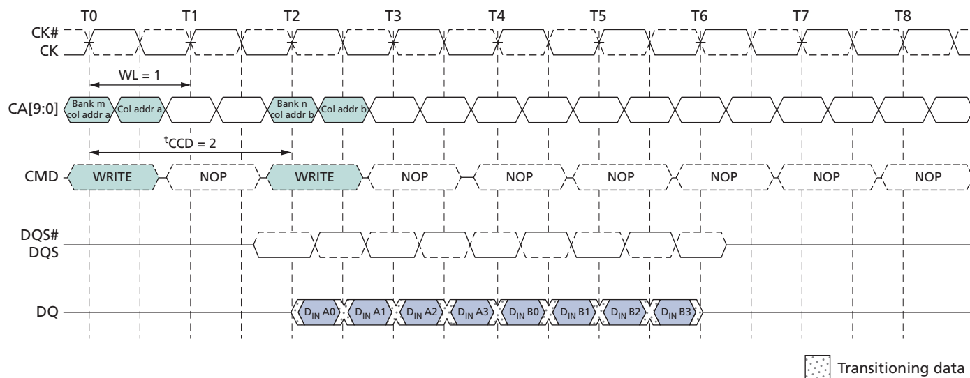
Figure 42: Seamless Burst WRITE – WL = 1, BL = 4, t_{CCD} = 2
