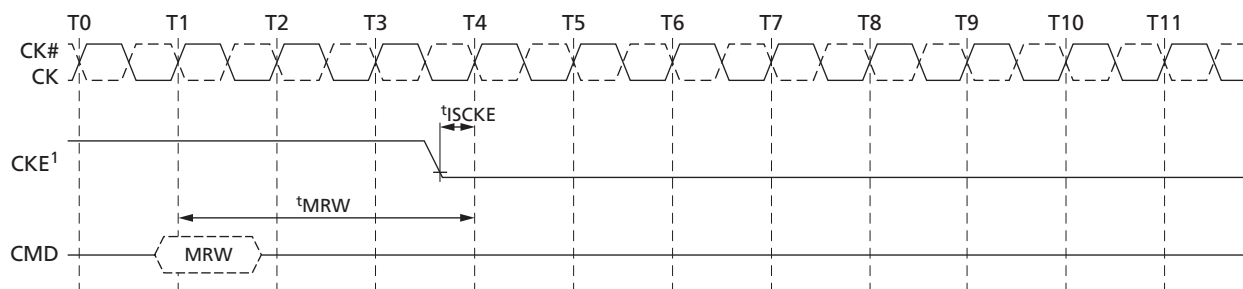
Figure 79: MRW Command to Power-Down Entry
