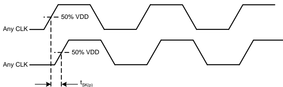
Figure 3. Output Skew
