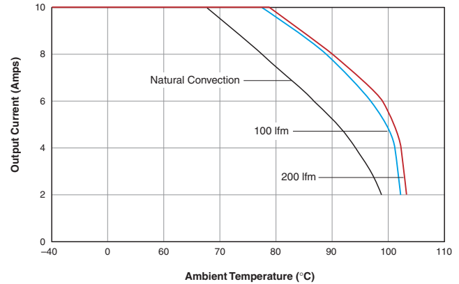
LSM-1.5/10-D3 Output Current vs. Ambient Temperature (SMT mount, air flow direction from pin 2 to pin 1)
