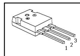
PG-TO247-3
