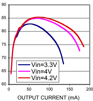
MIC2295 15V output Efficiency
