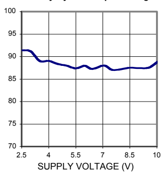
Max Duty Cycle vs Input Voltage
