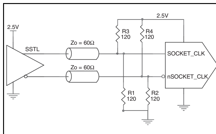
Figure 4B. SSTL Interface for V_{DD}/2 = 1.25V with No Available
