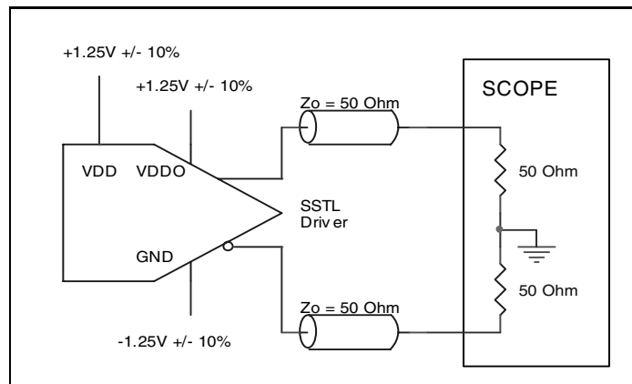
2.5V Core/2.5V Output Load AC Test Circuit
