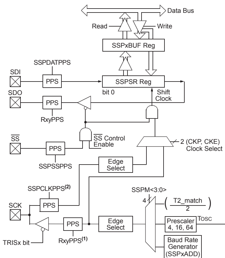
FIGURE 32-1: MSSP BLOCK DIAGRAM (SPI MODE)
