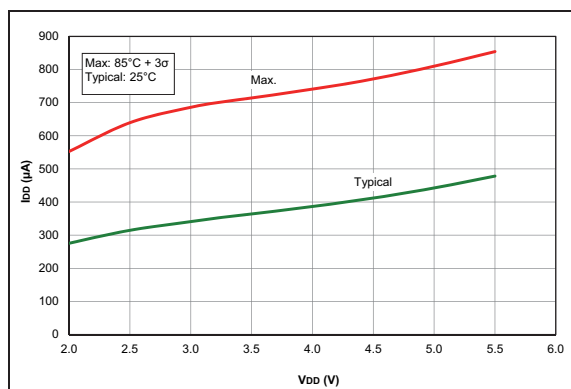
FIGURE 37-40: I_D , Op Amp, High GBWP Mode ( OPAxSP = 1 ), PIC16LF1764/5/8/9 Only.
