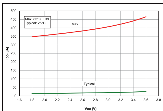
FIGURE 37-41: I_D , ADC Non-Converting, PIC16LF1764/5/8/9 Only.
