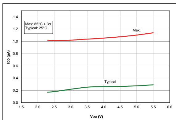
FIGURE 37-42: I_D , ADC Non-Converting, PIC16LF1764/5/8/9 Only.
