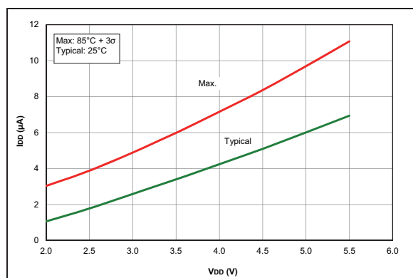
FIGURE 37-38: I_D , Timer1 Oscillator, F_{OSC} = 32\text{ kHz} , PIC16LF1764/5/8/9 Only.
