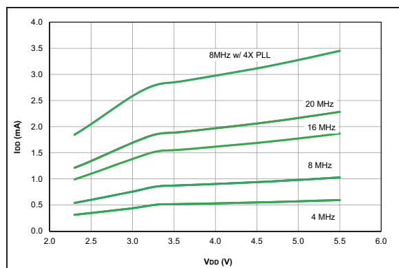
FIGURE 37-25: I_{DD} Typical, HS Oscillator, 25^\circ\text{C} , PIC16F1764/5/8/9 Only.
