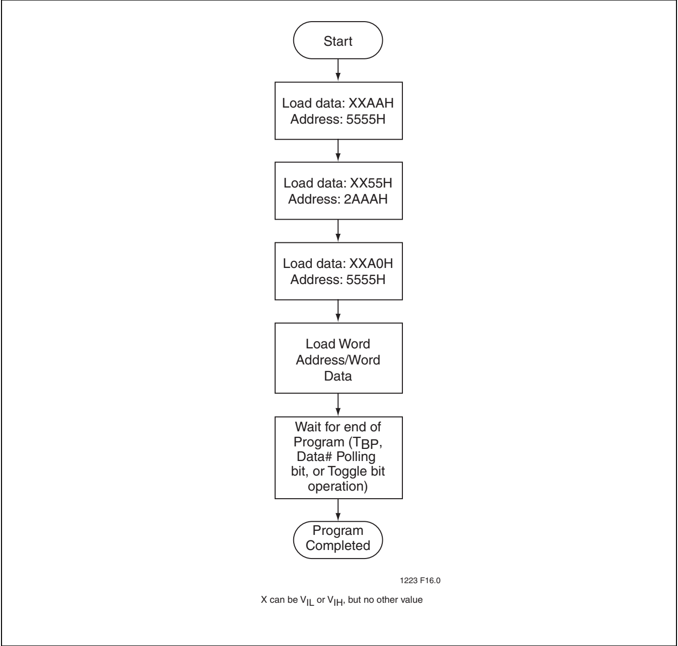
FIGURE 20: Word-Program Algorithm
