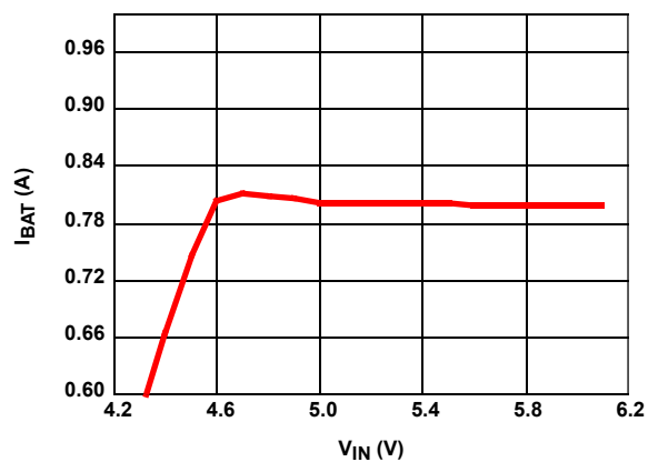
FIGURE 8. CHARGE CURRENT vs INPUT VOLTAGE
