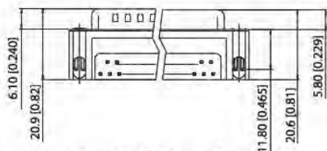
9.4mm[0.37"] Footprint
