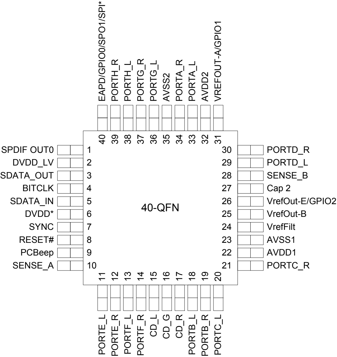
Figure 16. Pin Assignment
