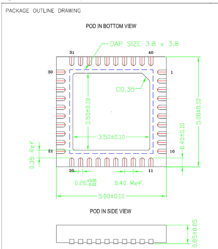
Figure 17. 40QFN Package Diagram
