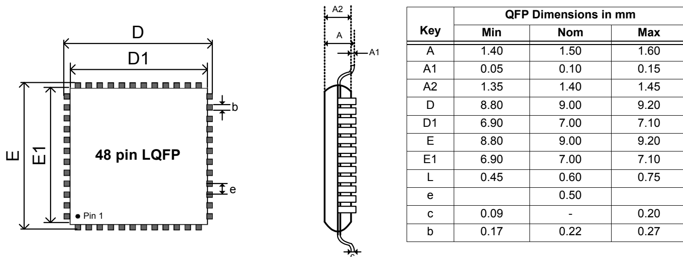
Figure 15. 48QFP Package Diagram
