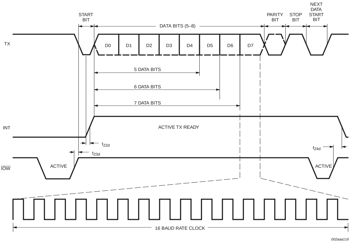
Fig 12. Transmit timing.
