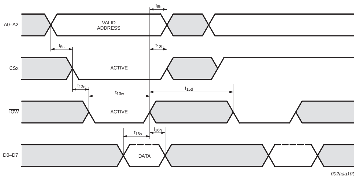
Fig 5. General write timing.
