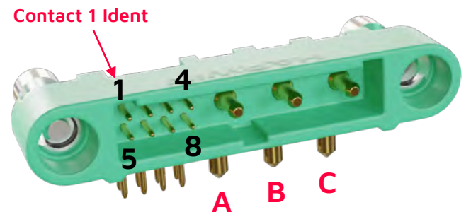
Male PCB mounted
