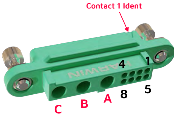
Female Crimp Housing
