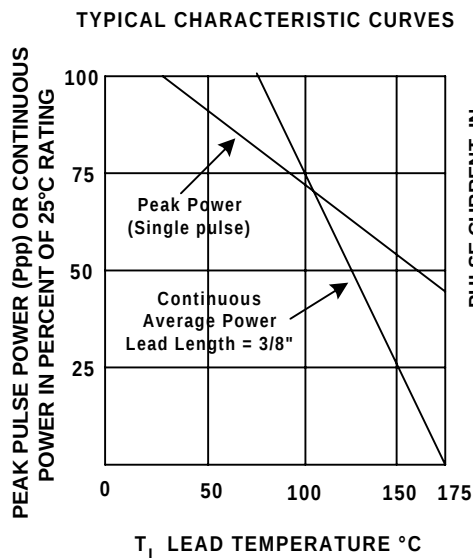
FIGURE 1 DERATING CURVE
