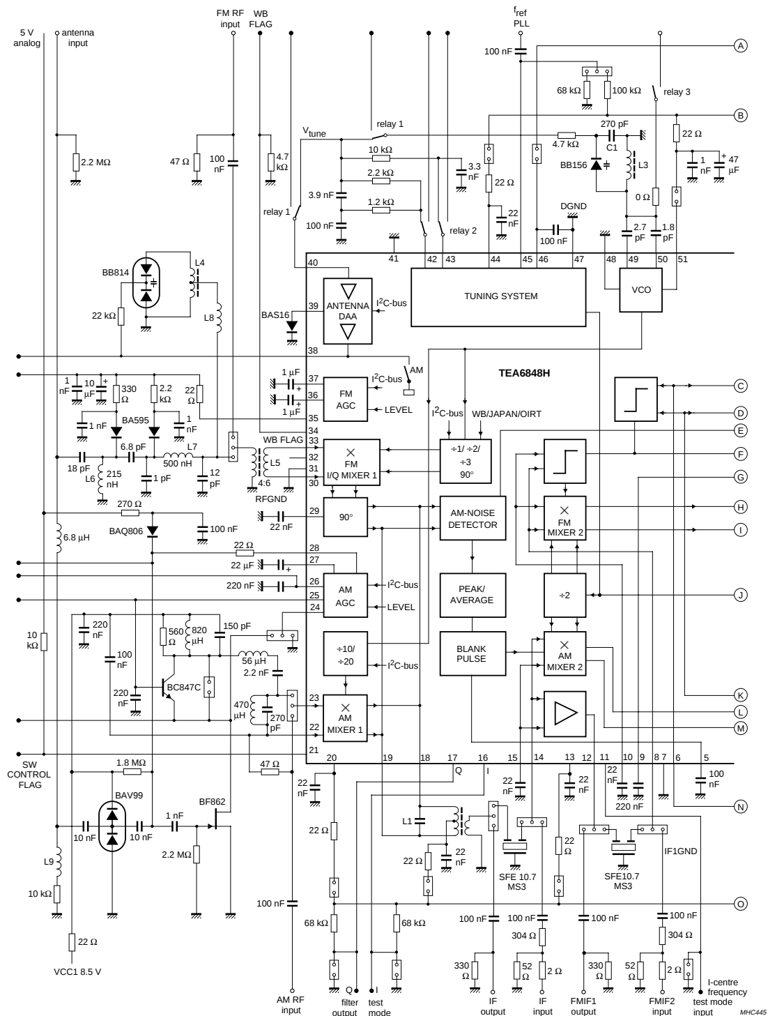
Fig.10 Test circuit (continued in Fig.11).
