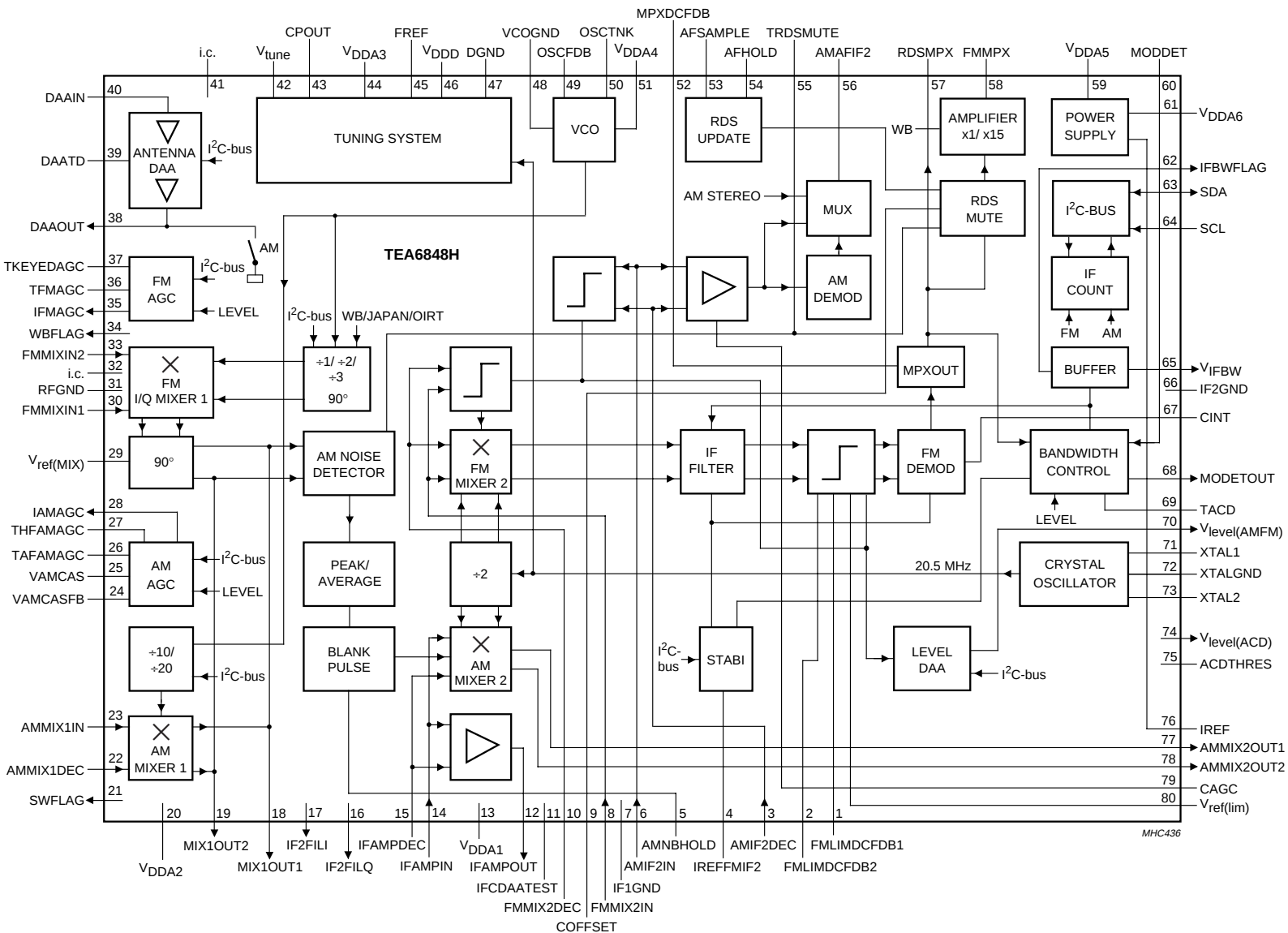
Fig.1 Block diagram.
