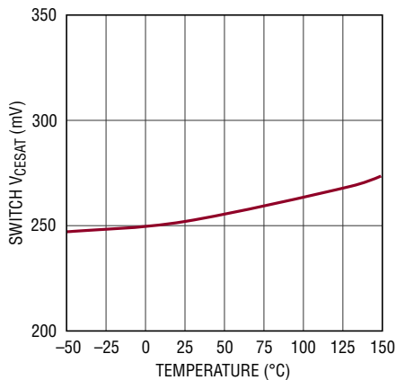
Switch V_{CESAT} ( I_{SW} = 500\text{mA} ) vs Temperature
