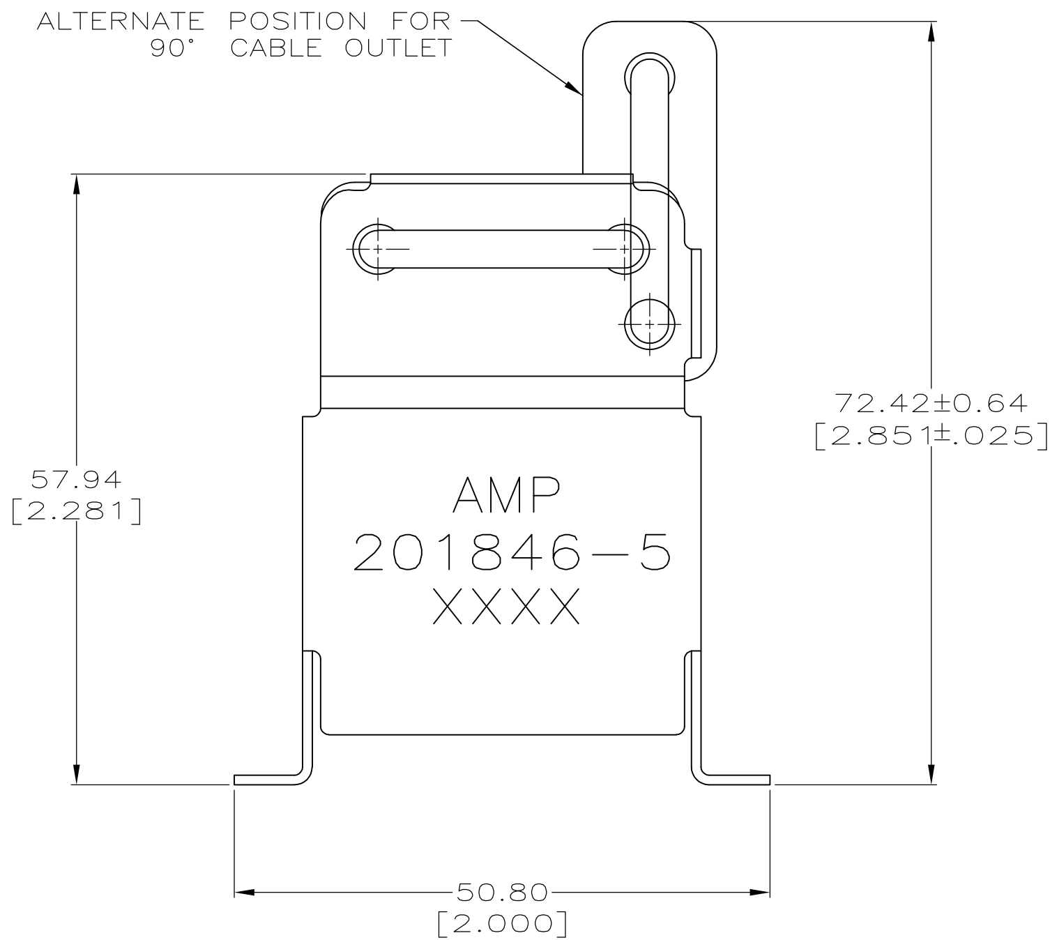
ASSEMBLED VIEW
