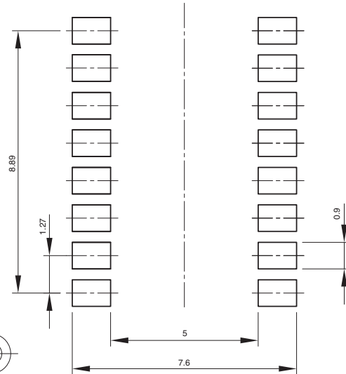
Possible footprint
