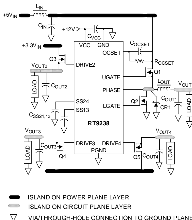
Fig.7 Layout Planning
