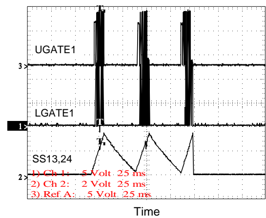
V_{OUT1} Short
