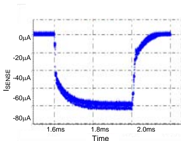
Fig.13 I_{SENSE} Current
