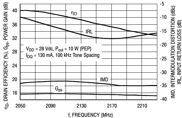
Figure 3. Two-Tone Wideband Performance @ P_{out} = 10 \text{ Watts (PEP)}
