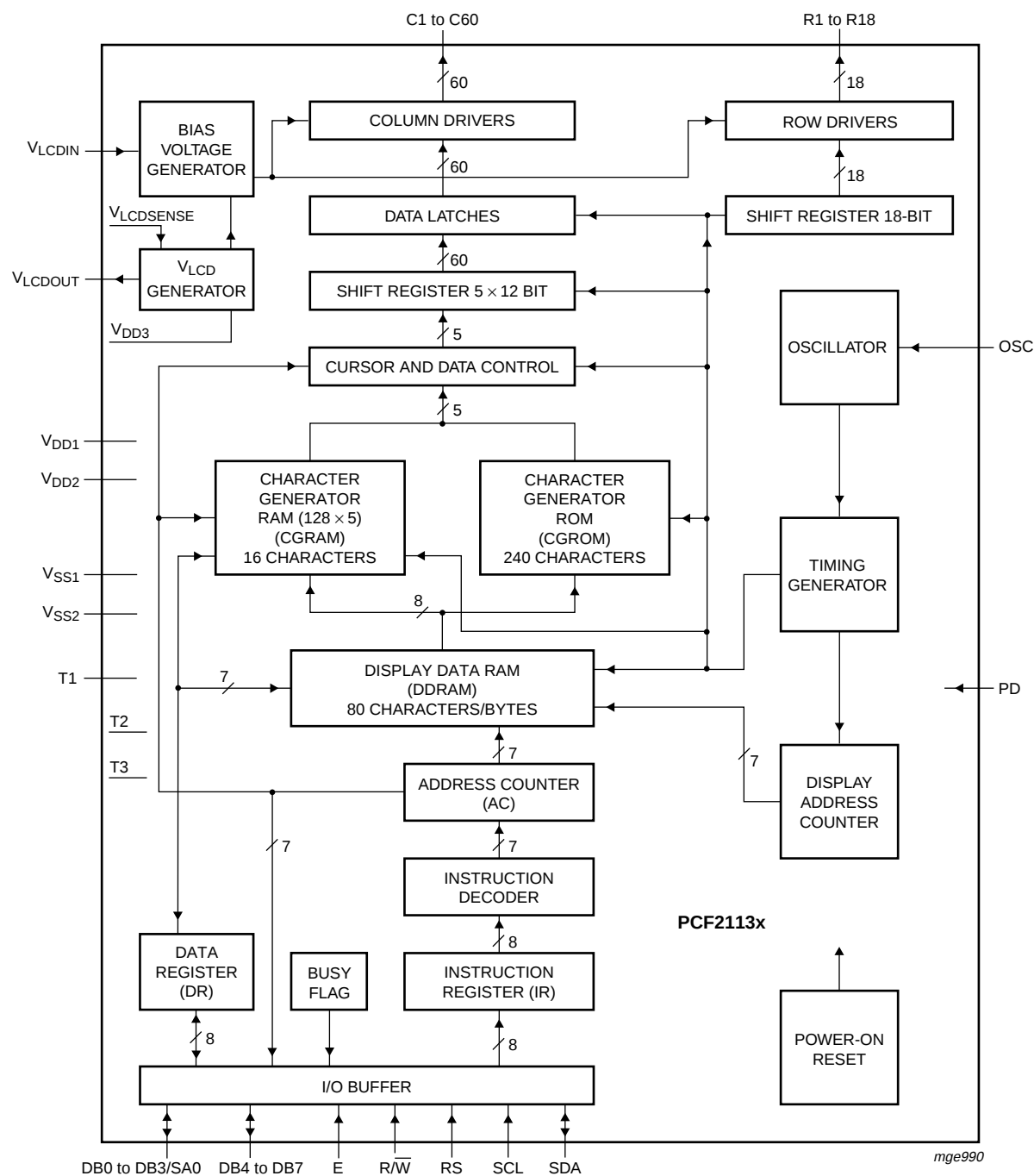
Fig 1. Block diagram of PCF2113x
