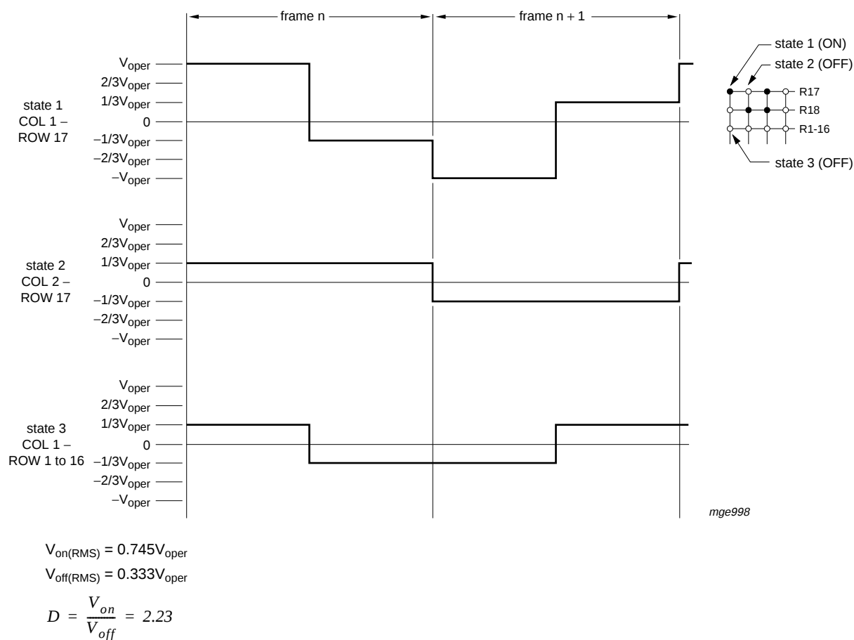
Fig 17. MUX 1:2 LCD waveforms; Icon mode (b)
