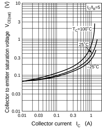
V_{CE(\text{sat})} - I_C
