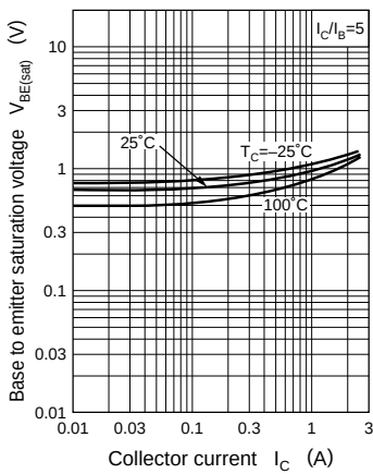
V_{BE(\text{sat})} - I_C
