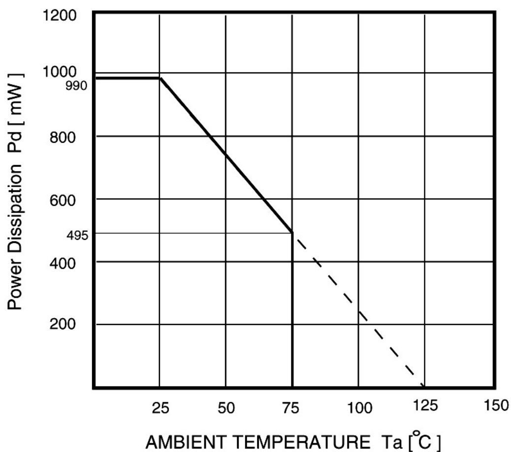
Thermal Derating
