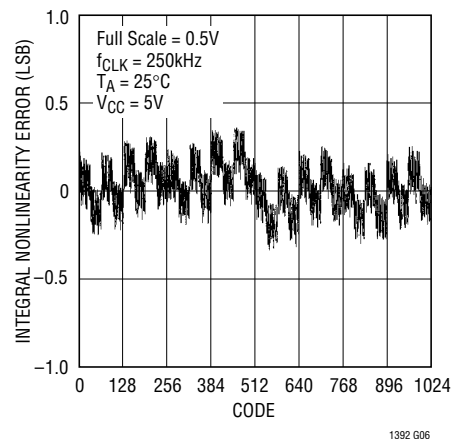
Integral Nonlinearity
