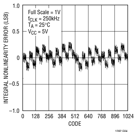
Integral Nonlinearity
