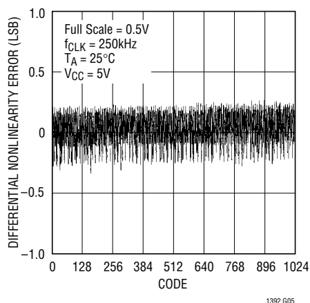
Differential Nonlinearity
