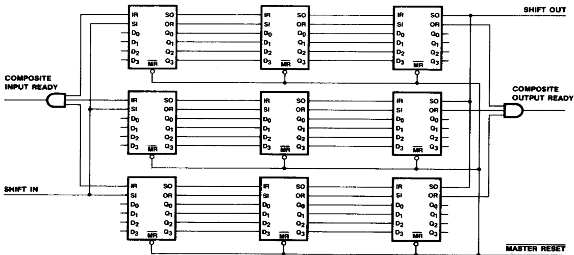
Figure 12. 192x12 FIFO with C5/C67401A/1
