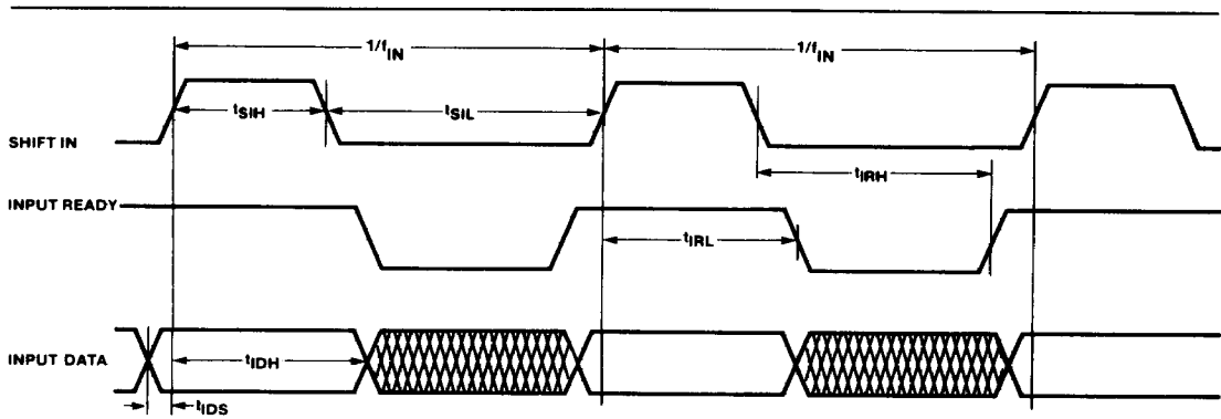
Figure 1. Input Timing
