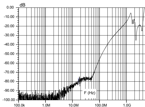
Figure 9. Analog crosstalk
