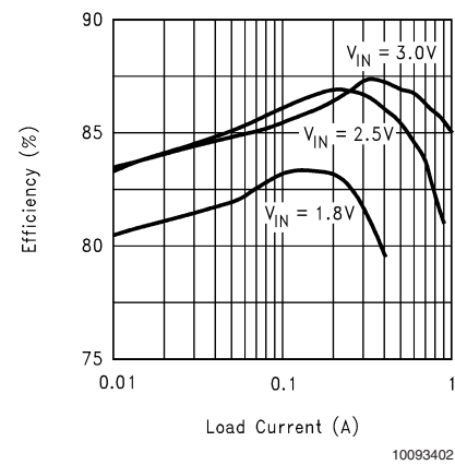
Efficiency vs Load Current V_{OUT} = 3.3V
