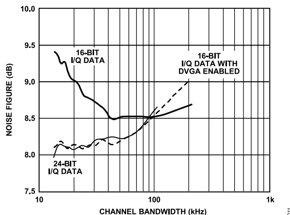
Figure 11. Noise Figure vs. Bandwidth (Minimum Attenuation, f_{CLK} = 13\text{ MSPS} )
