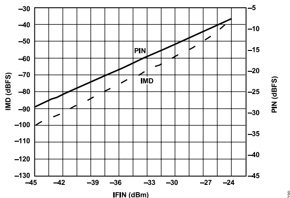
Figure 20. IMD vs. IFIN ( f_{CLK} = 18\text{ MSPS} )
