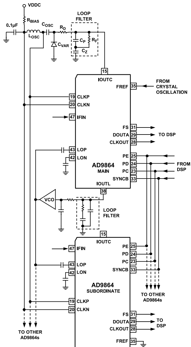
Figure 74. Example of Synchronizing Multiple AD9864 Devices
