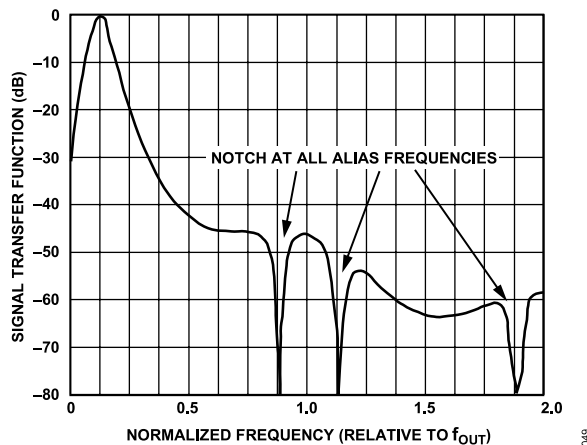
Figure 49. Signal Transfer Function of the Band-Pass \Sigma - \Delta Modulator from 0 f_{CLK} to 2f_{CLK}
