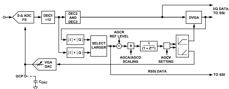
Figure 59. Functional Block Diagram of VGA and AGC
