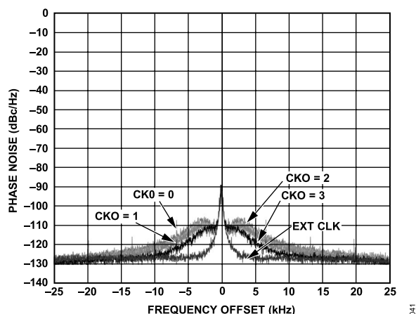
Figure 42. CLK Phase Noise vs. I_{BIAS} Setting (CKO); IF = 73.35 MHz, f_{IF} = 71.1\text{ MHz} , IFIN = -31\text{ dBm} , f_{CLK} = 18\text{ MHz} , f_{REF} = 16.8\text{ MHz} ; CLK SYN Settings: CKI = 7 , CLR = 56 , and CLN = 60 with f_{REF} = 300\text{ kHz}
