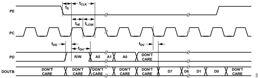
Figure 31. 4-Wire SPI Read Operation Timing
