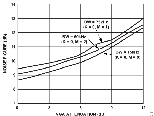
Figure 16. Noise Figure vs. VGA Attenuation ( f_{CLK} = 18\text{ MSPS} )
