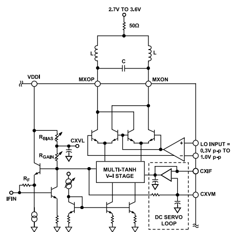
Figure 44. Simplified Schematic of AD9864 LNA/Mixer
