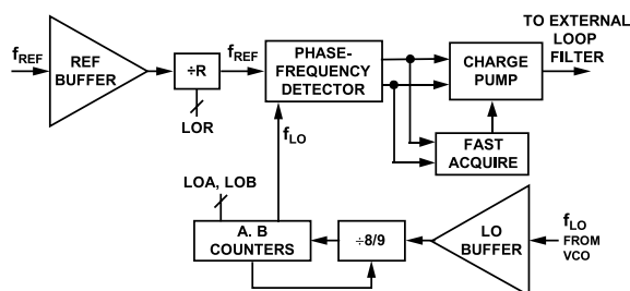
Figure 39. LO Synthesizer
