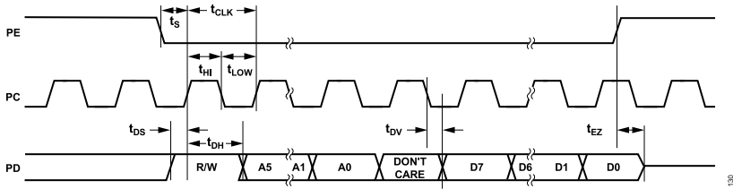
Figure 30. 3-Wire SPI Read Operation Timing
