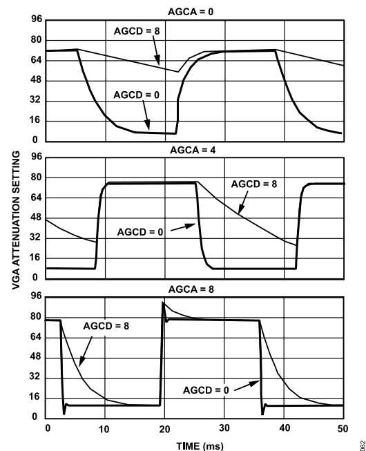
Figure 62. AGC Response for Different AGCA and AGCD Settings with f_{CLK} = 18 MSPS, f_{CLKOUT} = 20 kSPS, Decimate by 900, and AGCO = 0
