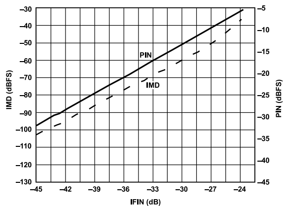
Figure 17. IMD vs. IFIN ( f_{CLK} = 13\text{ MSPS} )
