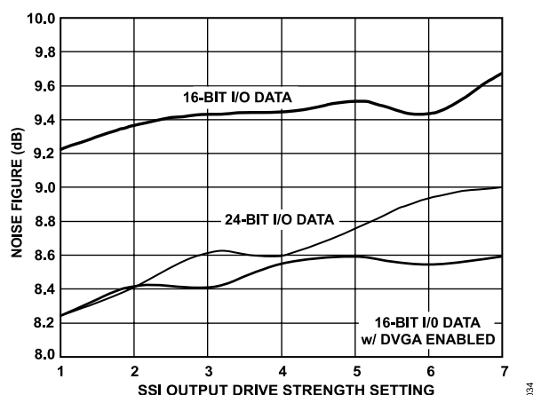
Figure 35. NF vs. SSI Output Drive Strength ( V_{DDx} = 3.0 V, f_{CLK} = 18 MSPS, BW = 10 kHz)
