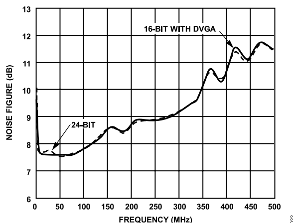
Figure 22. Noise Figure vs. Frequency (Minimum Attenuation, f_{CLK} = 26\text{ MSPS} , BW = 10\text{ kHz} )
