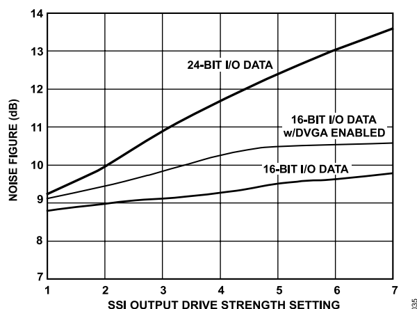
Figure 36. NF vs. SSI Output Drive Strength ( V_{DDx} = 3.0 V, f_{CLK} = 18 MSPS, BW = 75 kHz)
