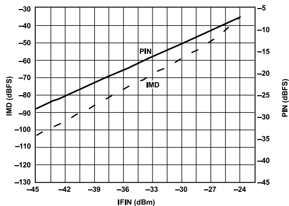
Figure 21. IMD vs. IFIN ( f_{CLK} = 26\text{ MSPS} )
