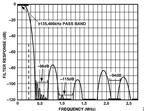
Figure 54. Decimation Filter Frequency Response for f_{OUT} = 541.666 kSPS ( f_{CLK} = 26 MHz, OSR = 48)
