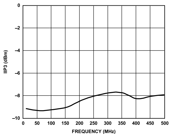
Figure 23. Input IIP3 vs. Frequency ( f_{CLK} = 26\text{ MSPS} )
