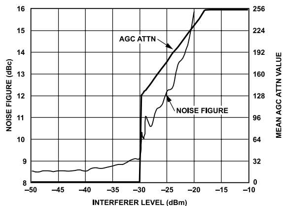
Figure 27. Noise Figure vs. Interferer Level (16-Bit Data with DVGA, BW = 12.5 kHz, AGCR = 1, f_{INTERFERER} = f_{IF} + 110\text{ kHz} )
