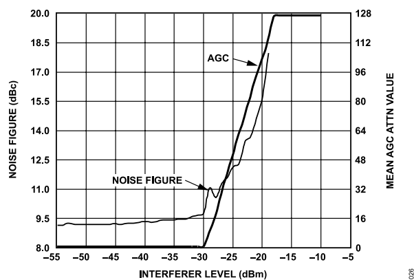
Figure 26. Noise Figure vs. Interferer Level (16-Bit Data, BW = 12.5\text{ kHz} , AGCR = 1 , f_{INTERFERER} = f_{IF} + 110\text{ kHz} )
