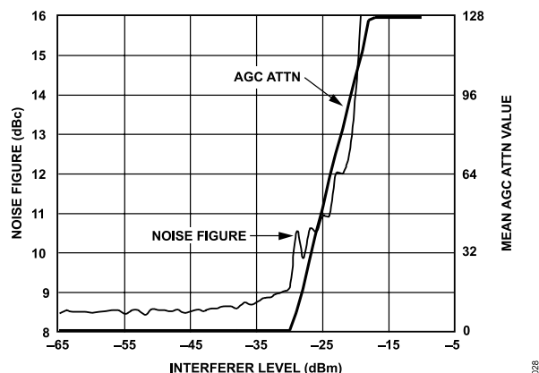
Figure 28. Noise Figure vs. Interferer Level (24-Bit Data, BW = 12.5 kHz, AGCR = 1, f_{INTERFERER} = f_{IF} + 110\text{ kHz} )
