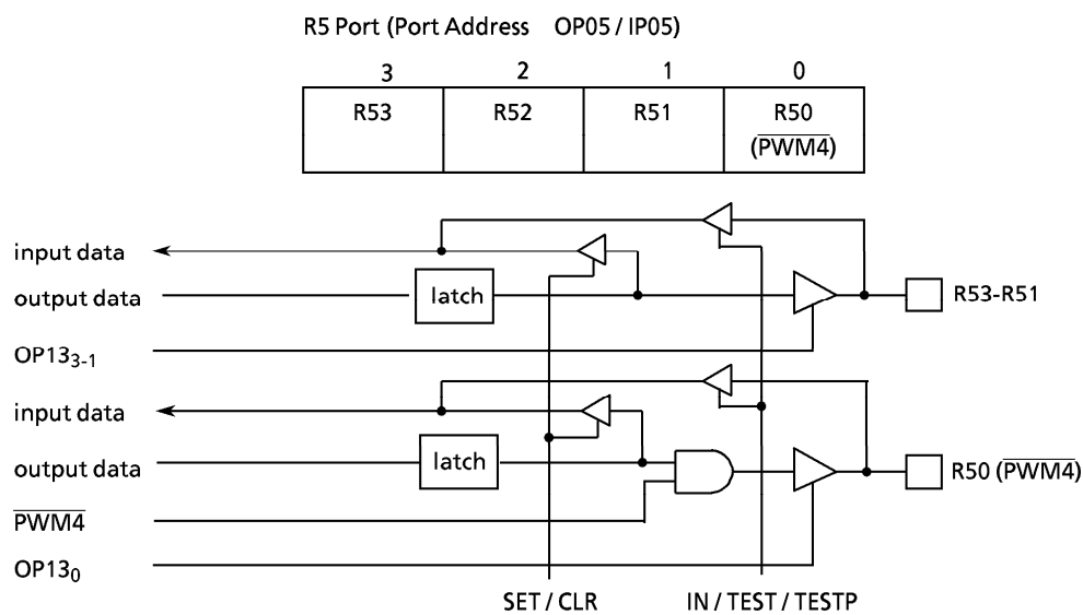
Figure 3-2. Port R5
