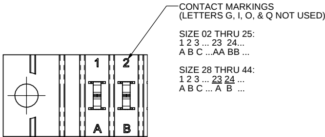
CONTACT ID SCALE 4:1
