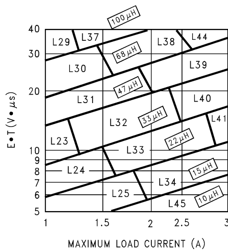
Figure 7-5. LM2670 – Adjustable
