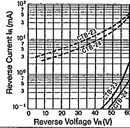
I_R - V_R Characteristics (Typical Value, per chip)
