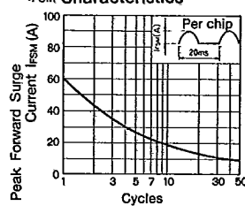
I_{FSM} Characteristics
