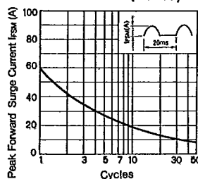
IFSM Characteristics (RK 13, 14)
