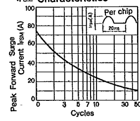
I_{FSM} Characteristics
