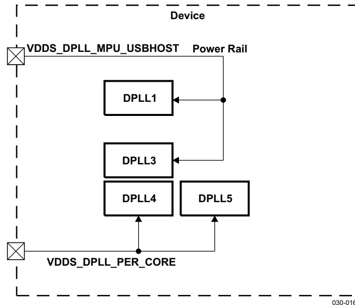
Figure 4-6. DPLL Implementation
