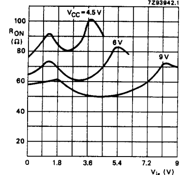
Fig.10 Typical ON-resistance ( R_{ON} ) as a function of input voltage ( V_{1S} ) for V_{1S} = 0 to V_{CC} - GND .
