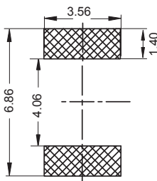
Recommended Layout for solder pads
