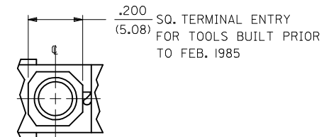
DETAIL "2"
