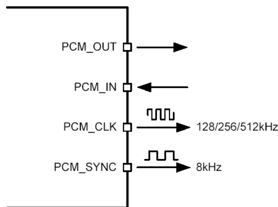
Figure 22: PCM Interface Master
