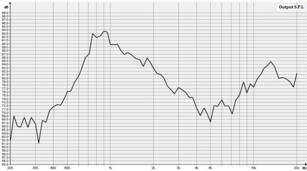
Frequency Response Curve (Fig. 2)
