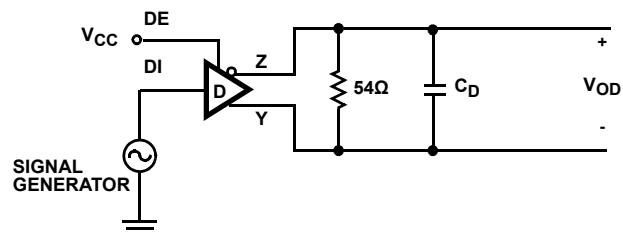
FIGURE 7A. TEST CIRCUIT
