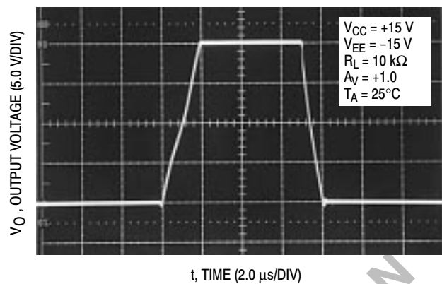
Figure 28. Transient Response
