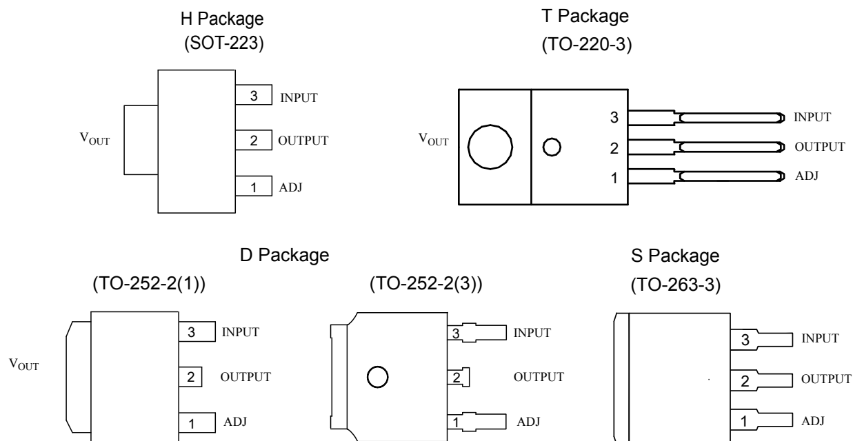
Figure 2. Pin Configuration of AZ317 (Top View)
