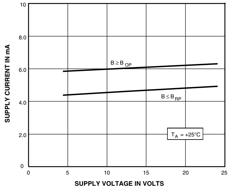
SUPPLY CURRENT
