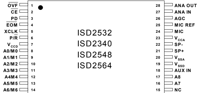
TSOP
