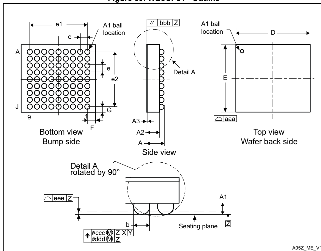
Figure 69. WLCSP81 - Outline
