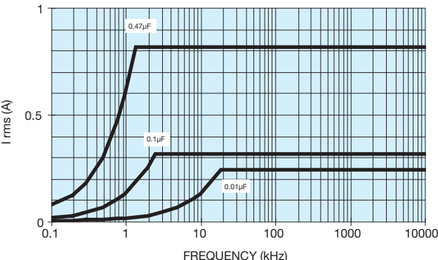
400 Vdc / 200 Vac
