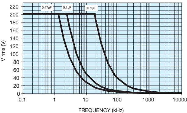
400 Vdc / 200 Vac
