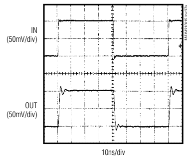
MAX4311 SMALL-SIGNAL PULSE RESPONSE
