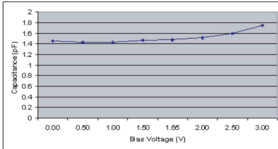
Figure 1. Typical Variation of C_{IN} vs. V_{IN} ( f = 1\text{ MHz} , V_P = 3.3\text{ V} , V_N = 0\text{ V} , 0.1\text{ }\mu\text{F} Chip Capacitor between V_P and V_N , T_A = 25^\circ\text{C} )
